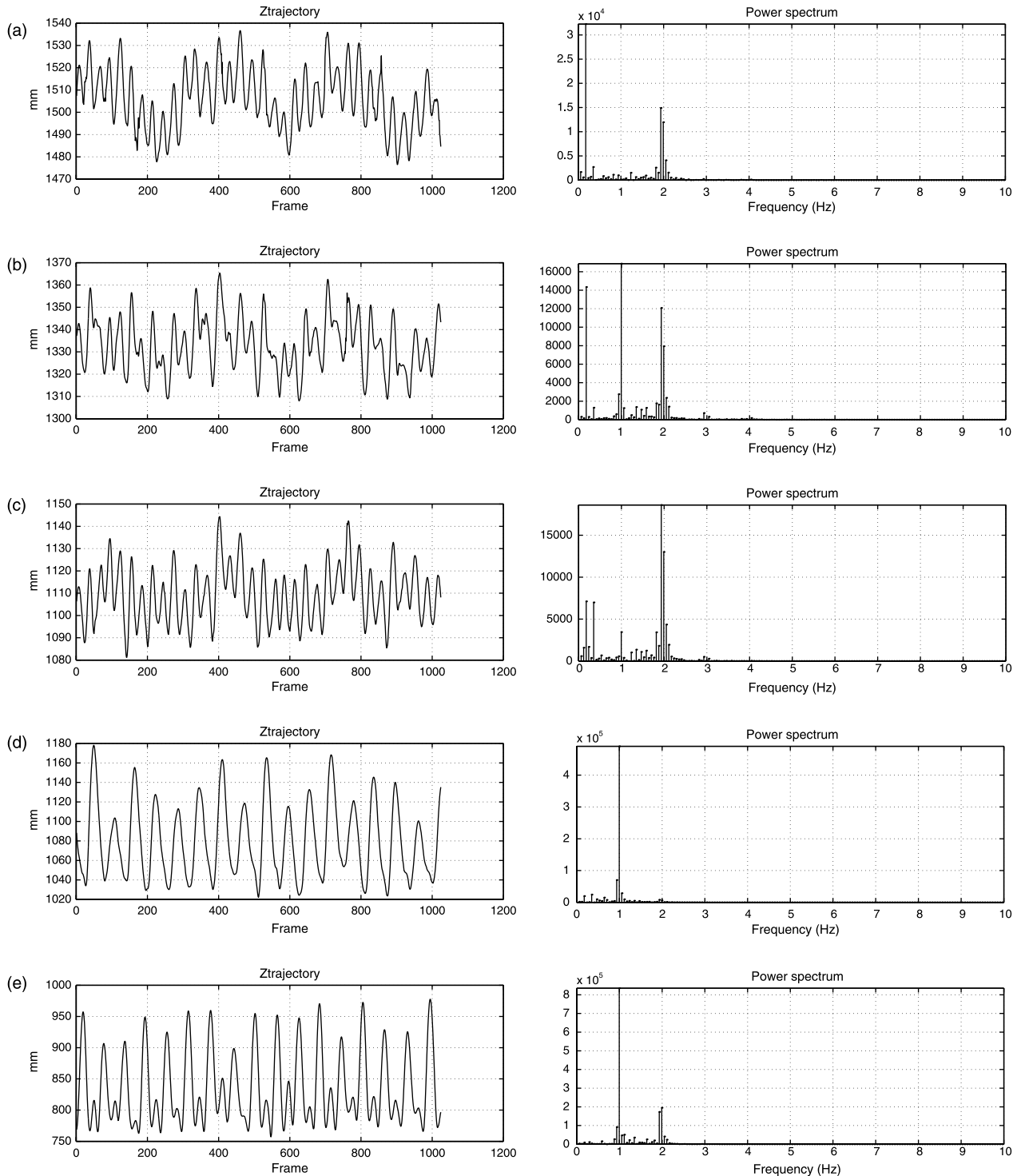
Fig. 3. Examples of vertical-component power spectra of a clockwise circle-walking person. N=1024 , f_s = 60 Hz, G_c=0.97 Hz.
