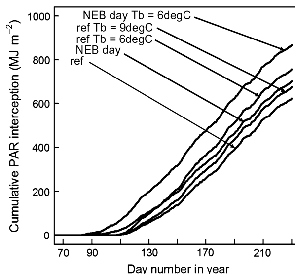
Fig. 11 The effect of changes in the start day for canopy expansion and of changes in base temperature for canopy expansion ( T_b ) on the cumulative PAR interception of Gig-311. The plots were produced by simulation using the model on Fig. 2 but with a T_b of 10 °C and its equivalent fitted LAI °C day -1 for Gig-311 of 0.01668. The other parameters were for Gig-311 from Tables 1 and 2. The reference line is for Gig-311 starting at the actual day when the canopy started to expand (stage FLL). The effect of decreasing the T_b value by 10% to 9 °C and to 6 °C but keeping all the remaining reference line parameterization the same are shown. The impact on the cumulative PAR interception of allowing the canopy to start expanding from the day when the buds first emerged (stage NEB) is also illustrated. Two such simulations are shown as follows: the first with the reference line parameterization but starting at the bud emergence day, and the second doing the same but with a T_b of 6 °C as well. The former shows that the leaf production should have been possible earlier in the year than was observed in the field.
