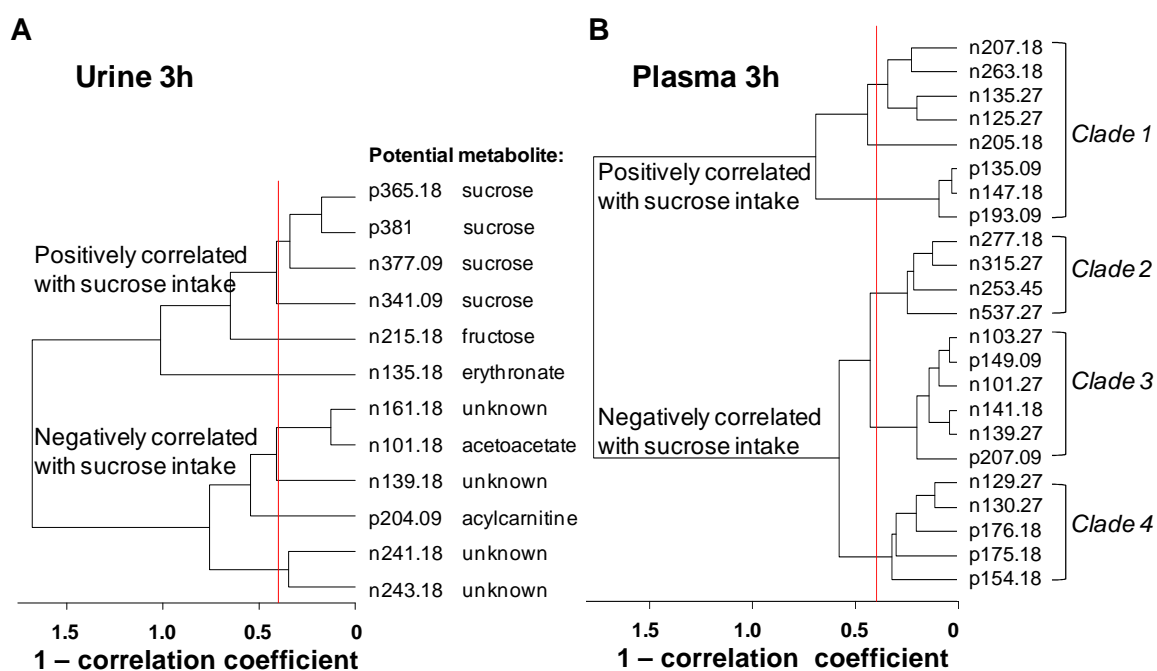
Figure 2. Hierarchical cluster analysis of Log 10 -transformed and TIC-normalized intensity values of putative metabolites discriminating between sucrose treatments in (A) 3 h urine (B) 3 h plasma samples with ions representing positive (p) and negative (n) ionisation mode features.
