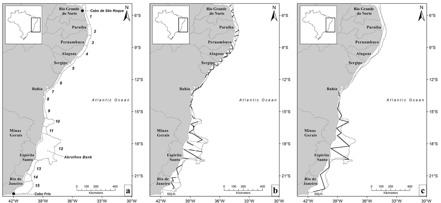
Fig 1. (a) Survey blocks to estimate the abundance of humpback whales off the Brazilian continental shelf, and (b) survey tracklines in 2008 and (c) in 2012. On-effort lines (black thick lines) overlap planned lines (grey dashed lines) in b and c.
