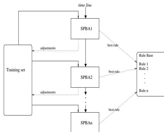
Figure 1: Iterative rule learning strategy
