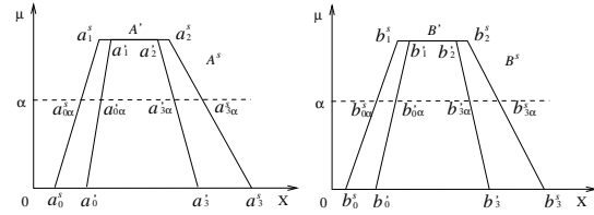
Figure 4: Preservation of piecewise linearity in scale transformation
