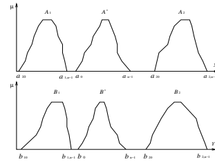
Figure 2: Interpolation with arbitrarily polygonal fuzzy membership functions
