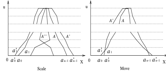
Figure 3: Scale and move transformations
