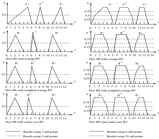
Figure 7: Examples of piecewise linearity for new HS method
