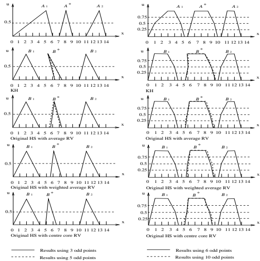
Figure 6: Examples of piecewise linearity for KH and original HS method
