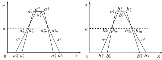
Figure 5: Preservation of piecewise linearity in move transformation
