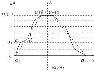
Figure 1: The RV of an arbitrary polygonal fuzzy set
