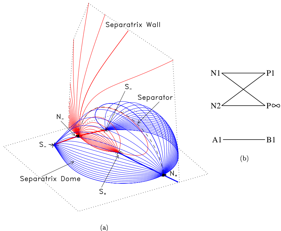
Figure 1: (a) 3D view of the intersecting topology: spines are thick lines, separatrix field lines are thin lines and the separator is a dashed line.
