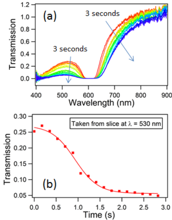
(Color Online) Figure 3; (a) Optical spectra taken from the pre-shear phase of an opal sample, showing the shear-melting of the crystal over 3 seconds. (b) Transmittance at \lambda = 530 nm as a function of shearing time. The points are fitted to a sigmoid function to extract a decay time.
