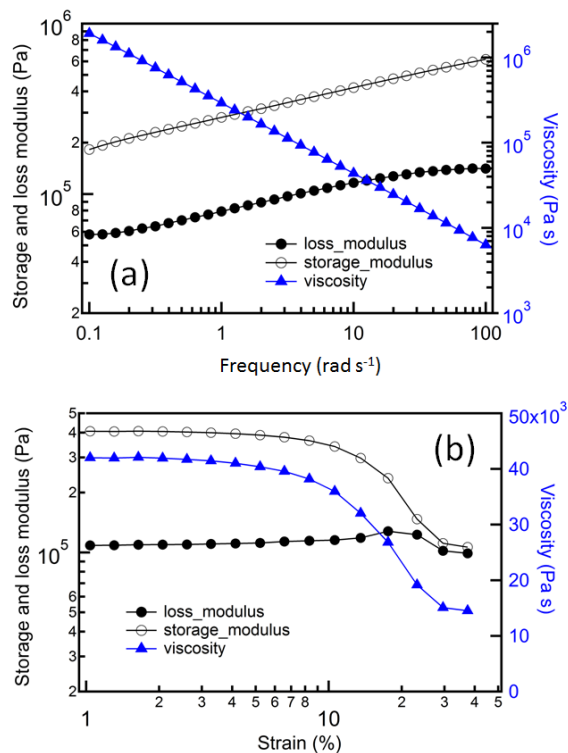
(Color Online) Figure 2 ; Storage & loss moduli, and the viscosity of polymer opal material, obtained using an ARES-G2 rheometer. Data is shown in (a) as a function of strain-shear oscillation frequency (temperature of 100°C), and in (b) as a function of strain magnitude (temperature of 100°C and an oscillation frequency of 10 rad/s). The polymer opal sample characterised here has a representative core-shell particle size of \approx 250\text{nm} , and T_{\text{glass}} \approx -15^\circ\text{C} .
