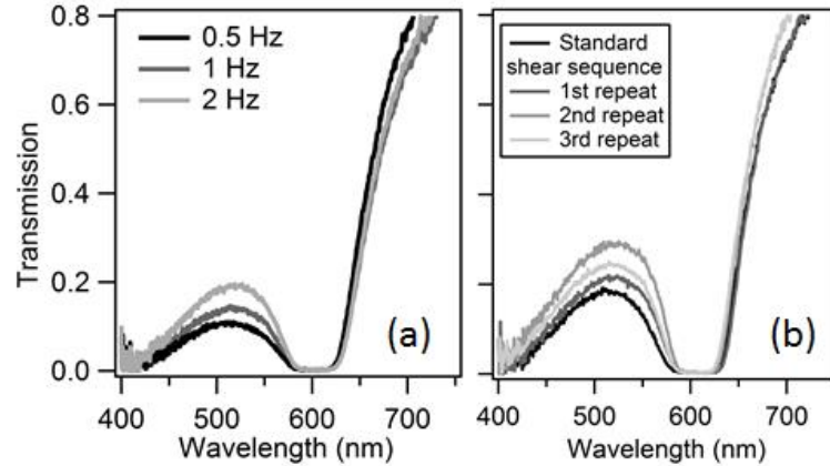
Figure 6; (a) Effect of variation of shear oscillation frequency on the end transmission spectrum, retaining other parameters from Table 1, and using a strain magnitude of 75%. (b) Spectra after multiple repetitions of the standard four-step shear sequence.
