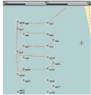
Figure 10: A map showing a survey pattern being followed using the cross track error minimization controller. The white circles around each waypoint indicate the threshold distance and the red line indicates the path taken.
