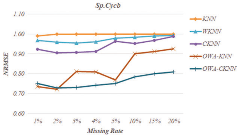
Figure 5: Method-specific NRMSE scores as averages from multiple trials, on the Sp.Cyca dataset
