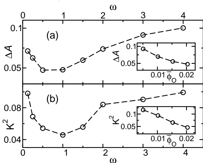
Fig. 4 (a) Excess surface area of the hydrophobic bilayer core plotted as a function of oil size. Inset shows excess surface area plotted against oil concentration for \omega = 1 . (b) Corresponding plots of the integrated squared curvature of the hydrophobic bilayer core.
