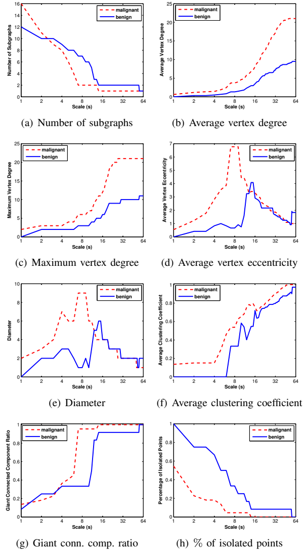
Fig. 4. The resulting eight graph feature sets extracted from the example malignant and benign microcalcification clusters in Fig. 1.
