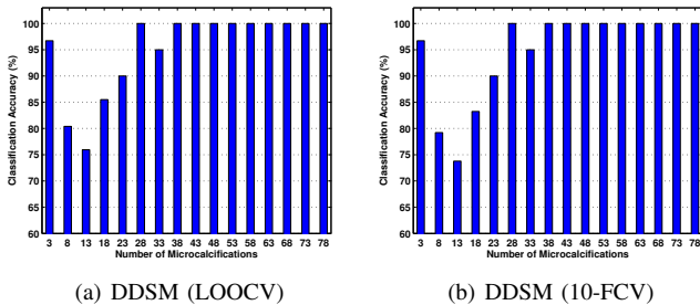
Fig. 7. Graph showing the classification accuracy as a function of the number of microcalcifications. The results are reported for the DDSM dataset using leave-one-out cross-validation (a) and 10-fold cross-validation (b) with the k NN classifier and S = 40 for leave-one-out cross-validation and S = 41 for 10-fold cross-validation.
