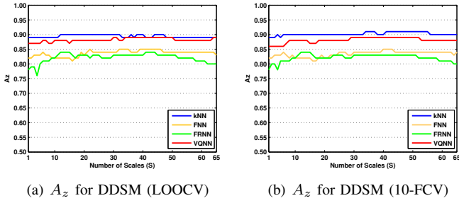
Fig. 5. The A_z values produced by the four classifiers for the DDSM dataset using leave-one-out (a) and 10-fold cross-validation (b).
