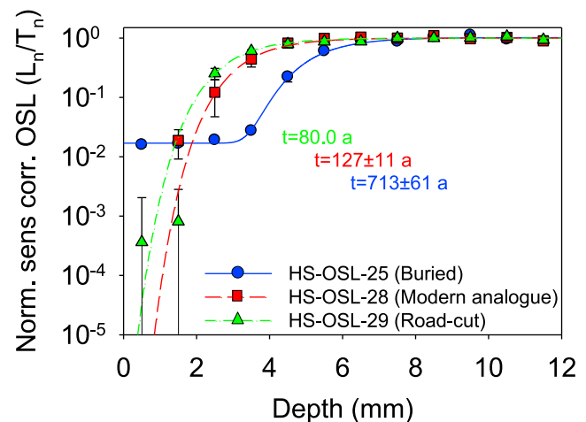
Figure 3. The same data as presented in Figure 2, but with L_n/T_n axis on a logarithmic scale. The finite signal built up in sample HS-OSL-25 during burial can be clearly seen.
