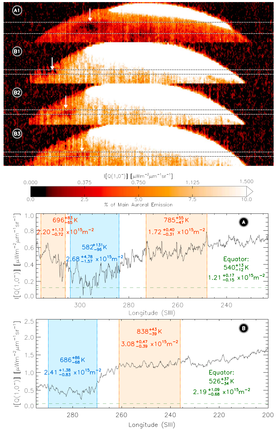
Figure 1. H 3 + emission measured by the CRILES on VLT. These observations were made on (a) 17 October and (b) 31 December 2012. Images of emission from the H 3 + v2 Q(1,0 - ) line, top, have been scaled to highlight subauroral emission, as shown by the color bar, and clearly show a region of darkening in the ionosphere (highlighted with arrows). The H 3 + emission from these images has been summed over the latitudinal region of the darkening (demarcated within the images by horizontal dotted lines), to produce two plots of varying H 3 + emission with system III longitude, bottom, one for 17 October and one for 31 December. Here the region of darkening can be clearly seen for both nights. We have calculated the mean temperature and column density, the two values displayed within each region, both inside the dark region (blue), and in the surrounding ionospheric regions (red). Using separate data, we have also calculated the mean equatorial emissions (dashed line), temperature, and column density for each night, measured within an hour of these observations (green).
