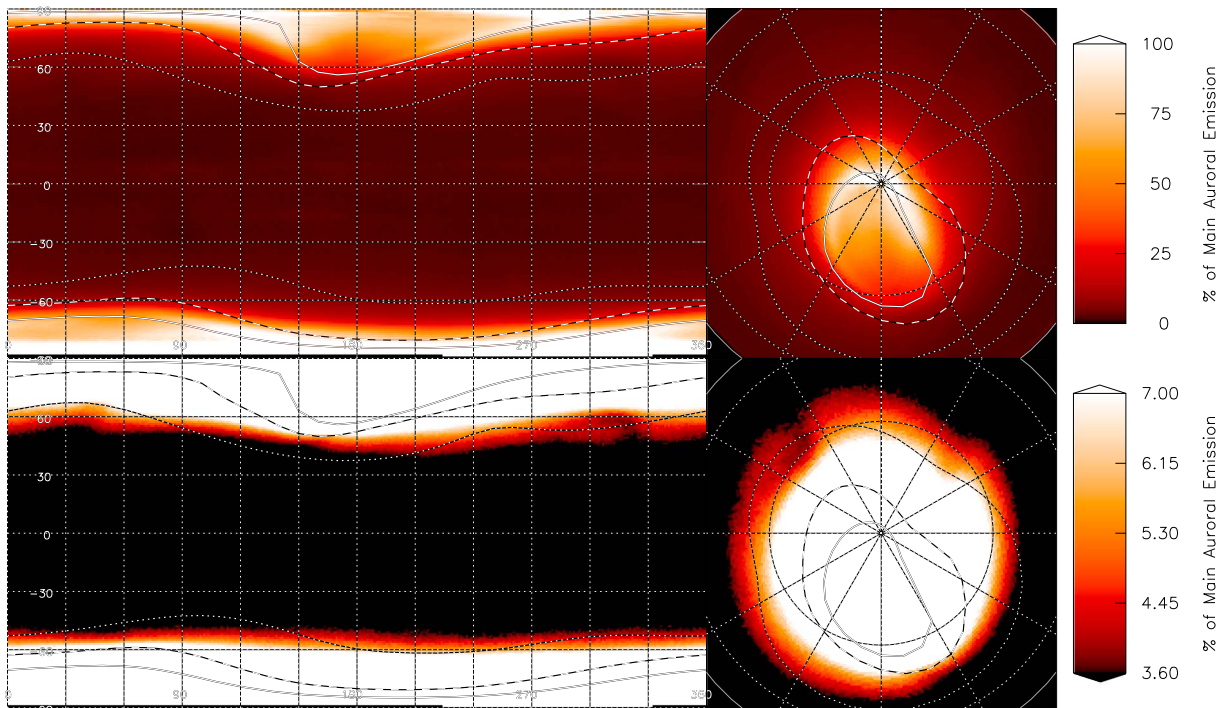
Figure 2. A map of mean H_3^+ emission across the 5 year Connerney and Satoh H_3^+ Jupiter image database. A latitude/longitude orthographic projection is shown on the left and a polar projection on the right. All maps show the emission scaled against the peak auroral brightness at latitudes between 75^\circ N and 75^\circ S with a gamma stretch of 0.5, and the bottom maps show a narrow range of emission brightness, scaled to highlight the subauroral region, as shown by the color bar. We identify the ionospheric locations that magnetically map to the main auroral emission (solid line; 30 R_J ) and Io spot and tail (dashed-line; 5.9 R_J ) [Grodent et al. , 2008], and to Amalthea (dotted line; 2.544 R_J ) [Connerney et al. , 1998]. Also shown are the jovigraphic longitude and latitude in 30^\circ steps (grey dotted line).
