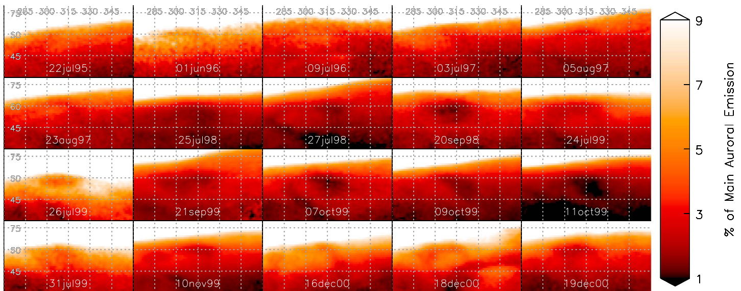
Figure 3. A clipped region of the latitude/longitude map ( 30\text{--}80^\circ N , 270\text{--}360^\circ W ), showing how emission from this region varies with time over the 1995–2000 period. Emission is scaled from the peak auroral brightness at latitudes between 75^\circ N and 75^\circ S with a gamma stretch of 0.5, to highlight the subauroral region, as shown in the color bar. Each frame has been smoothed by 2^\circ of latitude and longitude, in order to improve the signal to noise ratio, and lines of 15^\circ of latitude and longitude are shown (grey dotted line). Between 1995 and 1997, there are significant variations in this region, but no clear spot, and from 1998 onward a clear dark region occurs within each of these images, evolving in location and morphology.
