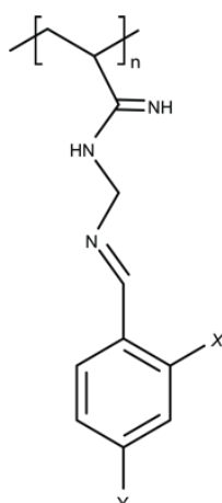
Figure 6. Polyacrylnitrilbenzaldehyde.
