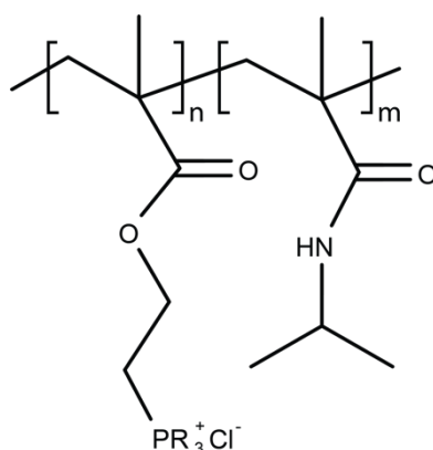
Figure 5. Polymer-containing phosphor-derivatives.
