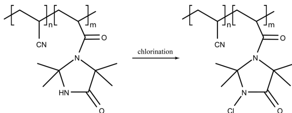
Figure 4. Chlorine-containing polymer.
