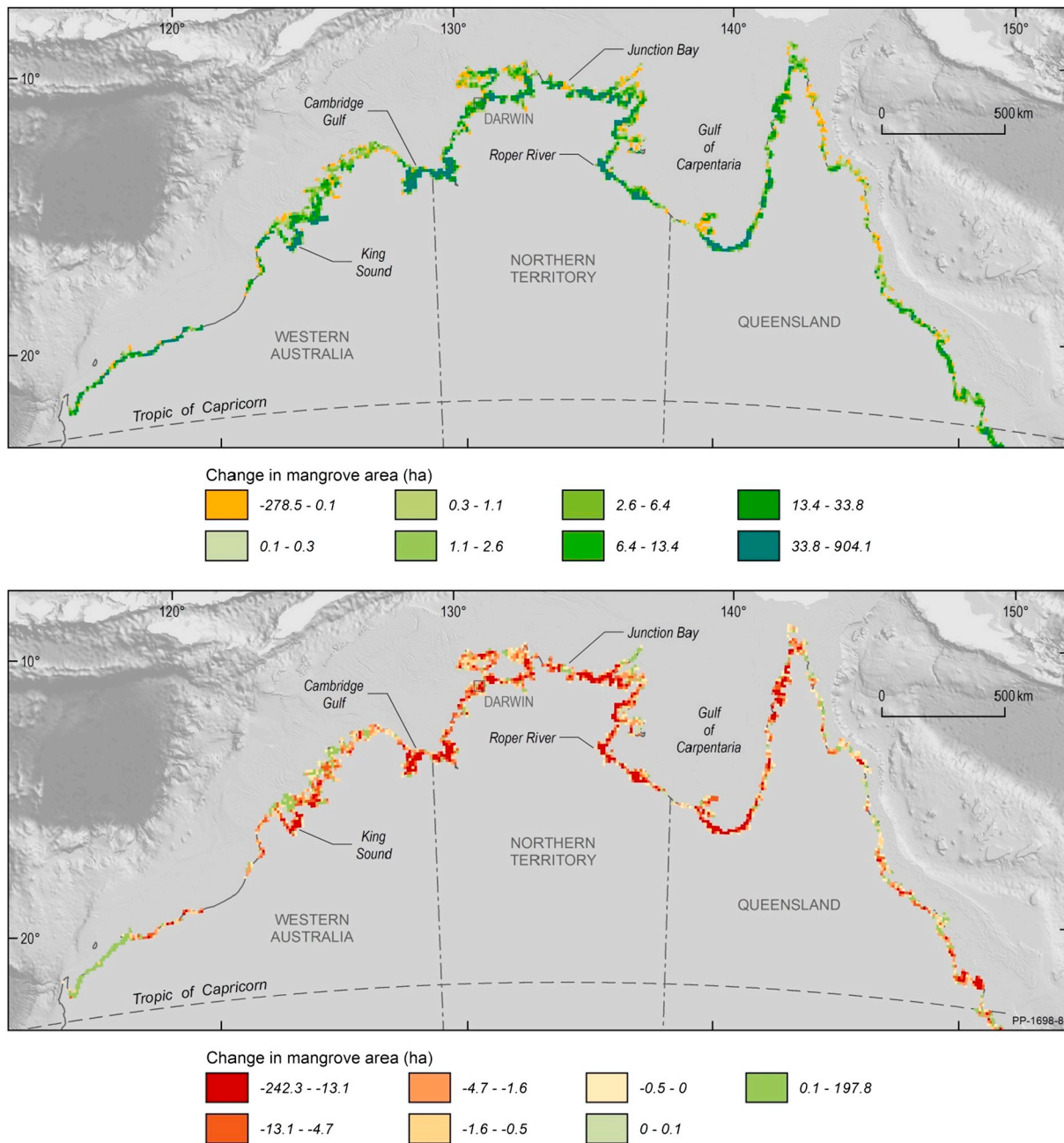
Fig. 10. a) Expansion of mangroves between 1994 and 2010 and b) decreases in mangrove extent between 2010 and 2016, with change in area shown for 10 × 10 km grid cells.
