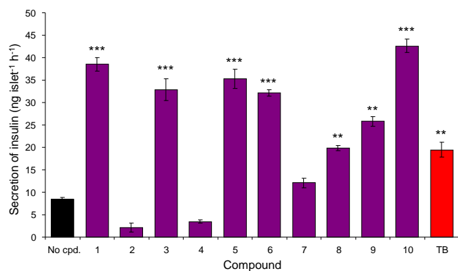
Figure 3. Glucose-stimulated secretion of insulin from murine pancreatic islets by compounds 1-10 . Freshly isolated islets were incubated for 1 h at 37°C in KRB buffer containing glucose (16.7 mM) in the absence (negative control) or presence of different test compounds and the amount of insulin secreted was measured. Values are mean \pm SEM from three independent experiments. ** p < 0.01 , *** p < 0.001 , compared with the value for the negative control. TB = tolbutamide.
