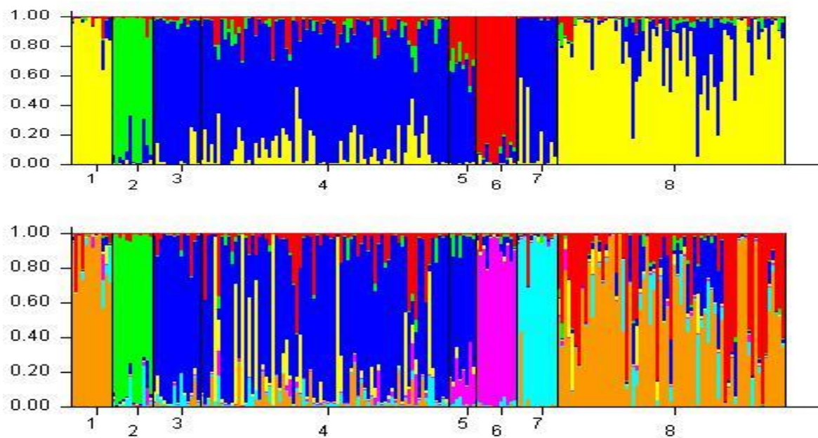
Figure 5: STRUCTURE plot for SNP data at k = 4 (top) and k = 7 (bottom)
