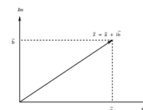
Fig. 1. A fuzzy complex number
