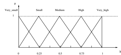
Fig. 2. Fuzzy quantity space for both certainty and fuzzy matching degrees
