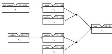
Fig. 3. Emerging scenario space after backward chaining initiated by e_1
