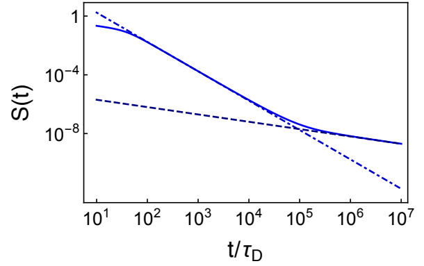
FIG. 1. Decay of the survival probability under quantum Brownian motion. The change in the power-law governing the survival probability of a pure initial Gaussian state (solid line) is shown in a log-log scale as a function of time in units of the decoherence time. The long-time asymptotic expressions for t \gg \tau_D in the two distinct regimes \gamma t \ll 1 (dotted-dashed line) and \gamma t \gg 1 (dashed line) are also shown, with \gamma = 10^{-3} and D\sigma^2 = 100 , with \hbar/m\sigma^2 as a unit of frequency.
