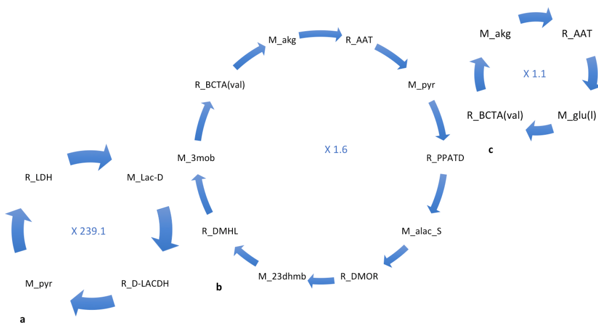
Figure 1. Cycles unique to phototrophic conditions in the mitochondrion: (a) pyruvate regeneration, (b) pyruvate recycling linked to 2-oxoglutarate recycling and (c) glutamate and 2-oxoglutarate cycling. Species starting with 'R_' indicate reactions whilst 'M_' indicate metabolites. Abbreviations: 23dhmb: 2,3-dihydroxy-3-methylbutanoate, 3mob: 3-methyl-2-oxobutanoate, AAT, alanine aminotransferase, alac_S: 2-acetolactate, BCTA(val): branched-chain-amino-acid transaminase (valine forming), akgl: 2-oxoglutarate, D-LACDH: D-lactate dehydrogenase, DMHL: 2,3-dihydroxy-3-methylbutanoate hydro-lyase, DMOR: 2,3-dihydroxy-3-methylbutanoate NADP + oxidoreductase (isomerizing), glu: Glutamate, lac-D: lactate; LDH: lactate dehydrogenase; PPATD: pyruvate acetaldehydetransferase (decarboxylating) pyr: pyruvate.
