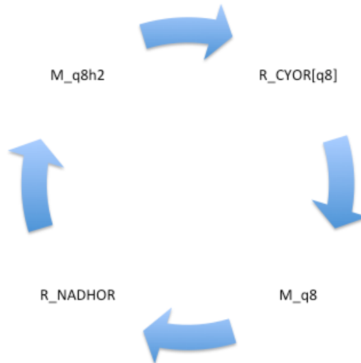
Figure 2. Mixotrophic cycle carrying the greatest mass flux within the mitochondrion. Species starting with 'R_' indicate reactions whilst those with 'M_' indicate metabolites. Abbreviations: q8: ubiquinone; q8h2: ubiquinol; NADHOR: ubiquinone oxidoreductase complex I; CYOR: ubiquinol-cytochrome c oxidoreductase complex III.
