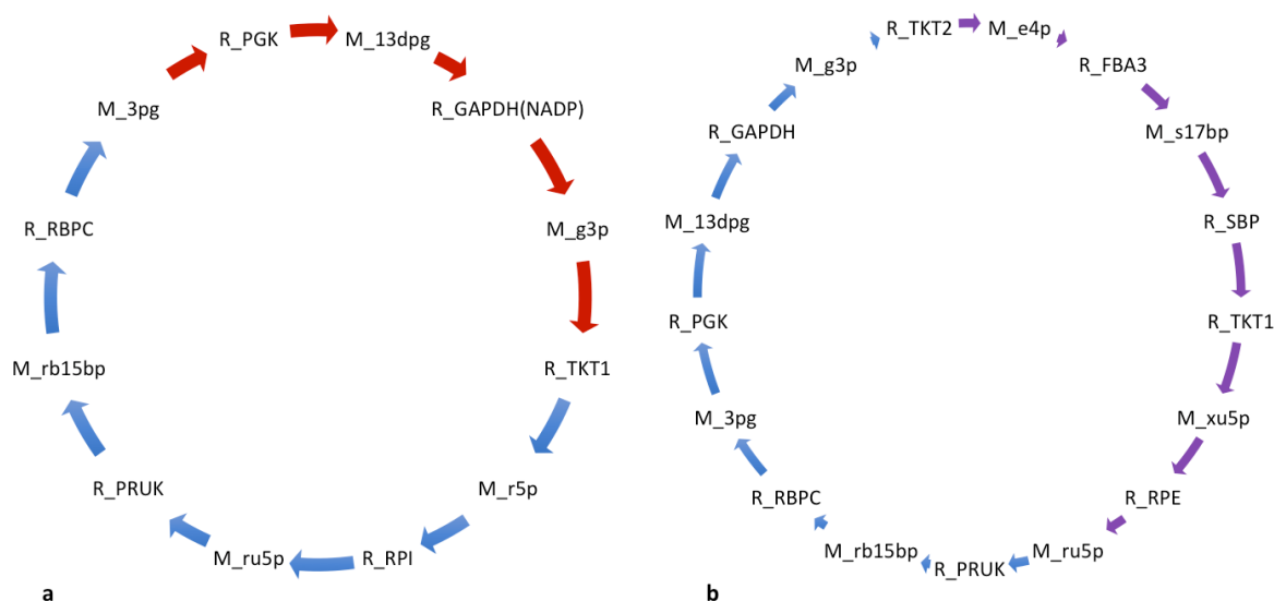
Figure 5. Unique cycles resulting from the mitochondrion, thylakoid lumen and chloroplast. (a) Phototrophic cycles included reactions of the Calvin-Benson cycle (blue arrows) and glycolysis (red arrows) whilst (b), mixotrophic growth resulted in the same Calvin-Benson cycle reactions (blue arrows) associated with the reactions of the pentose phosphate pathway (purple arrows). Species starting with 'R_' indicate reactions whilst 'M_' denotes metabolites. Abbreviations: 13dpg: 3-phospho-D-glyceroyl phosphate; 3pg: 3-phospho glycerate; e4p: erythrose 4-phosphate; FBA3: sedoheptulose 1,7-bisphosphate D-glyceraldehyde-3 phosphate lyase; g3p: glyceraldehyde 3-phosphate; GAPDH: glyceraldehyde 3 phosphate dehydrogenase; GAPDH(NADP): glyceraldehyde 3 phosphate dehydrogenase (NADP+); PGK: phosphoglycerate kinase; PRUK: phosphoribulokinase; r5p: ribose 5-phosphate; RBPC: ribulose-bisphosphate carboxylase; rb15bp: ribulose 1,5-bisphosphate; RPE: ribulose-5-phosphate 3-epimerase; RPI: ribose-5-phosphate isomerase; ru5p: ribulose 5-phosphate; s7p: sedoheptulose 1,7-bisphosphate; s17bp: sedoheptulose 1,7-bisphosphate; TKT1: transketolase 1; TKT2: transketolase 2; xu5p: xylulose 5-phosphate.
