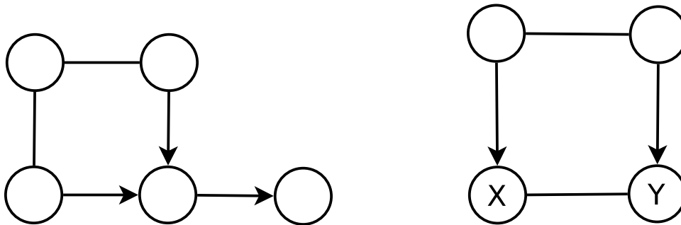
Figure 4: V-Structures
