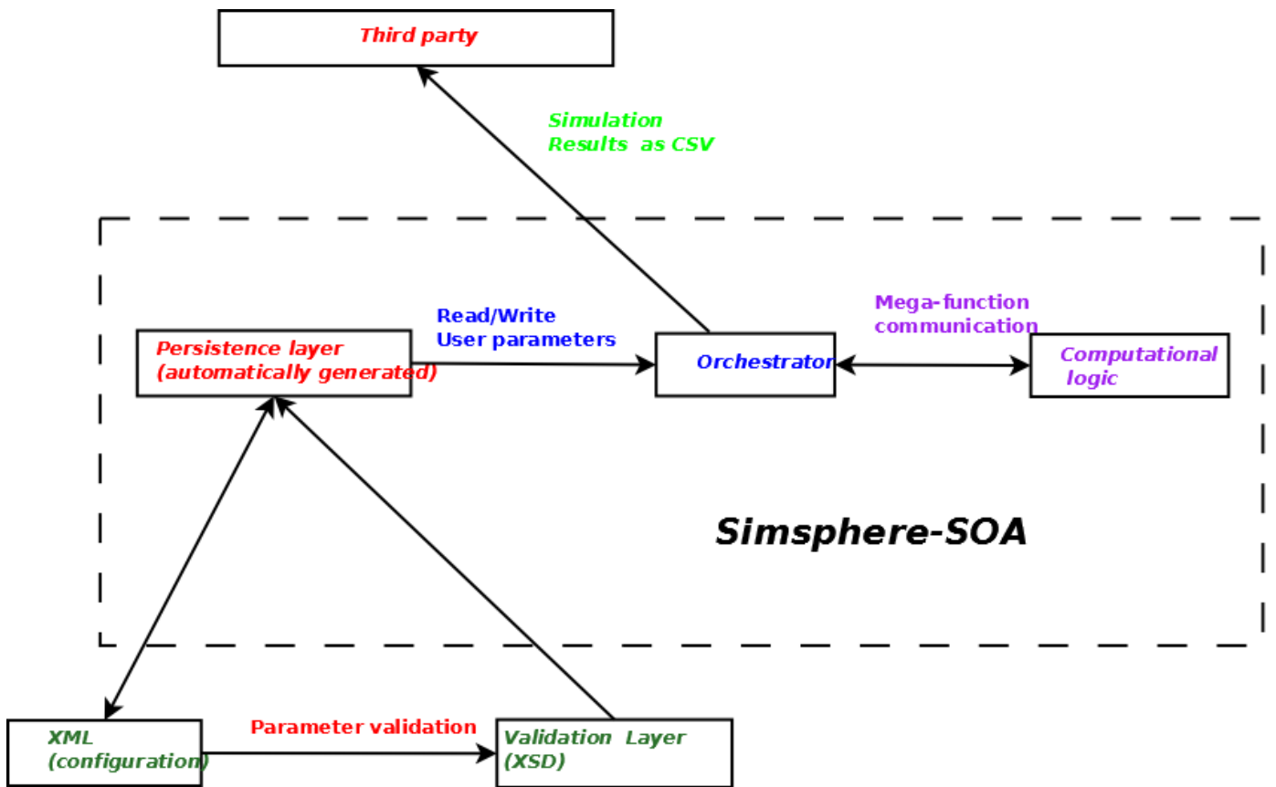
Fig. 3 The new friendly architecture of SimSphere-SOA
