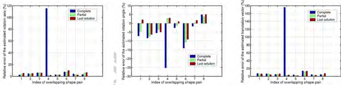
Figure 7: Relative errors of the estimated rotation axis (Left), rotation angle (Middle), and translational vector (Right) of our RBAB method using different schemes for the fusion of the underlying transformations estimated by different weak estimators. The overlapping shape pair index from 1 to 8 refers to duck0–40, frog40–80, dinosaur144–180, tubby120–160, bird100–60, cow42–45, peach280–240, and lobster60–80 respectively.
