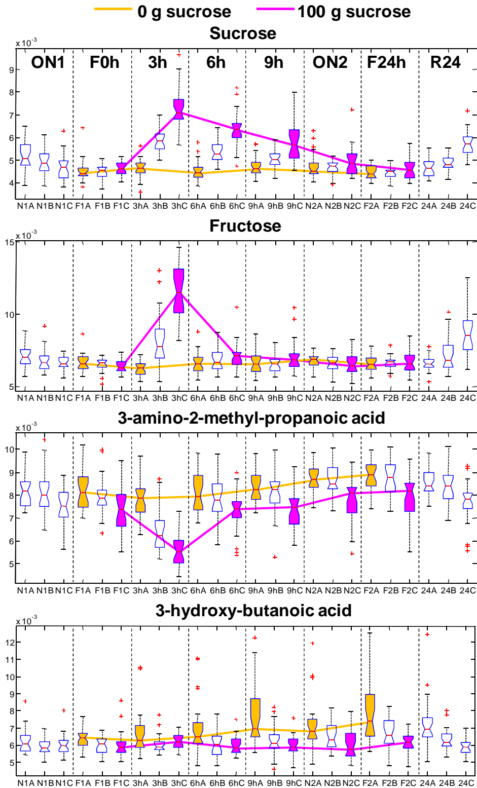
Figure 5. Log10-transformed intensity values of sucrose, fructose, 3-amino-2-methyl-propanoic acid and 3-hydroxy-butanoic acid discriminating between sucrose treatment: repartitioning of urine Gas Chromatography –time-of-flight - Mass Spectrometry (GC-tof-MS) data by meta-class sampling time and treatment. Sampling times post sucrose intake are shown; ON, overnight urine collections; F, fasting; R, reconstituted 24 h urine sample.
