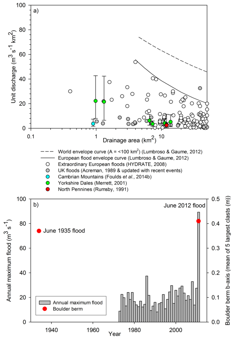
Figure 10. (a) Unit discharge of extreme upland floods based on geomorphological data, plotted alongside other UK and European data; (b) annual maximum flow and boulder-berm data for the Afon Leri (Wales).
