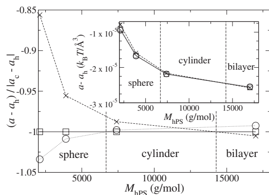
FIG. 5. The inset shows the free energy density predicted by SCFT for blends of the symmetric copolymer SB 20/20 with a range of homopolymers. The free energy density is measured with respect to that of the homogeneous blend with the same weight fraction of copolymer and is plotted against homopolymer molecular weight. In all cases, copolymer has 12.5 wt %. The main panel shows the same data normalized with respect to the magnitude of the free energy density of a cylindrical micelle. The free energy density of this morphology then appears as a horizontal line and the corresponding data for the lamella and sphere approach it from above and below. The data for the spherical micelle are plotted as circles connected by dotted lines. Those for the cylinder are plotted as squares linked by full lines and those for the lamella are shown as crosses connected by dashed lines. The vertical dashed lines mark the approximate boundaries between the different morphologies.
