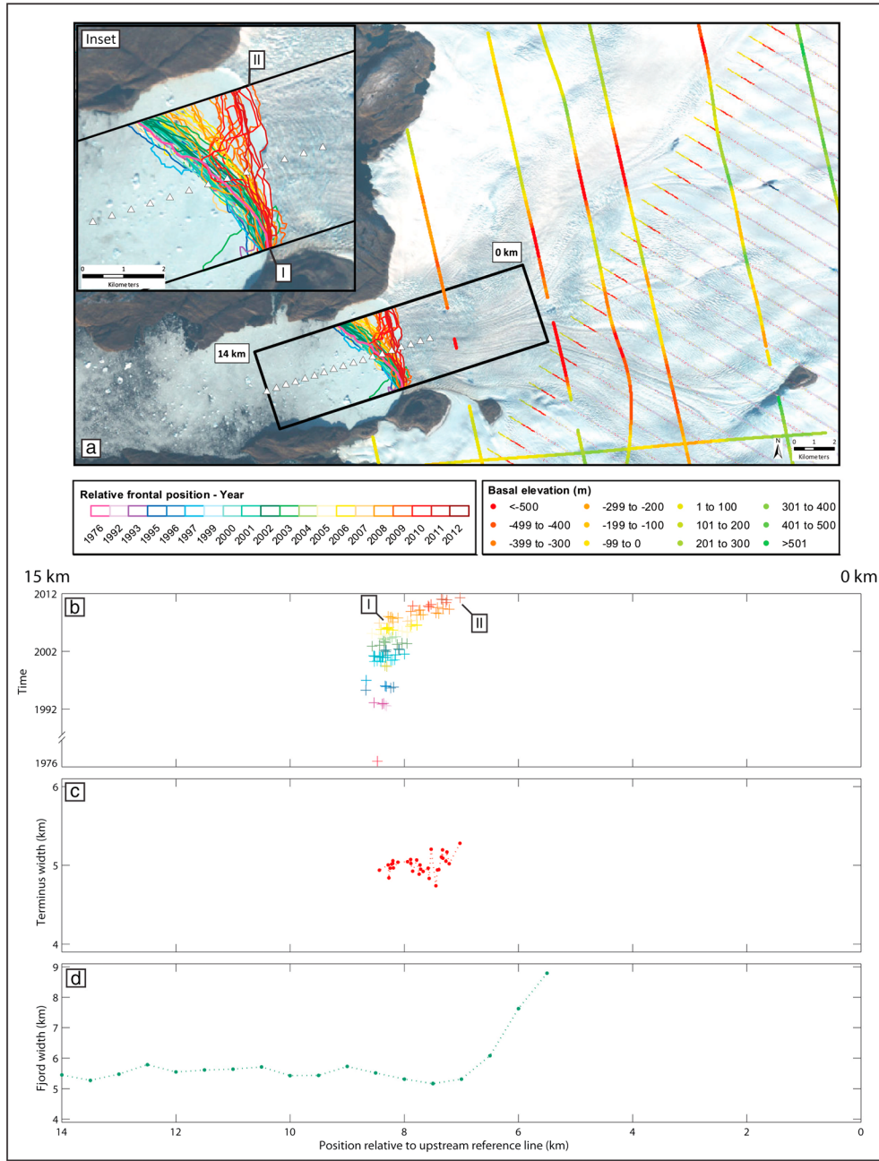
Figure 6. Frontal position of Igdgludlip Sermia in relation to basal elevation, fjord width parallel to the glacier terminus, and fjord width perpendicular to the centerline. (a) IGD frontal position over time (colored lines) in to ice-bottom elevations from CReSIS radar depth sounder flightlines, color coded from green (high elevation) to red (low elevation). Labeled positions are discussed in the text. Base image: Landsat scene acquired 11 September 2011 and provided by USGS GLOVIS. (b) IGD frontal position over time (colored crosses), relative to upstream reference line. (c) Fjord width parallel to the glacier terminus, for each available frontal position. (d) Fjord width perpendicular to the centerline (sample locations indicated by white triangles in Figure 6a).
