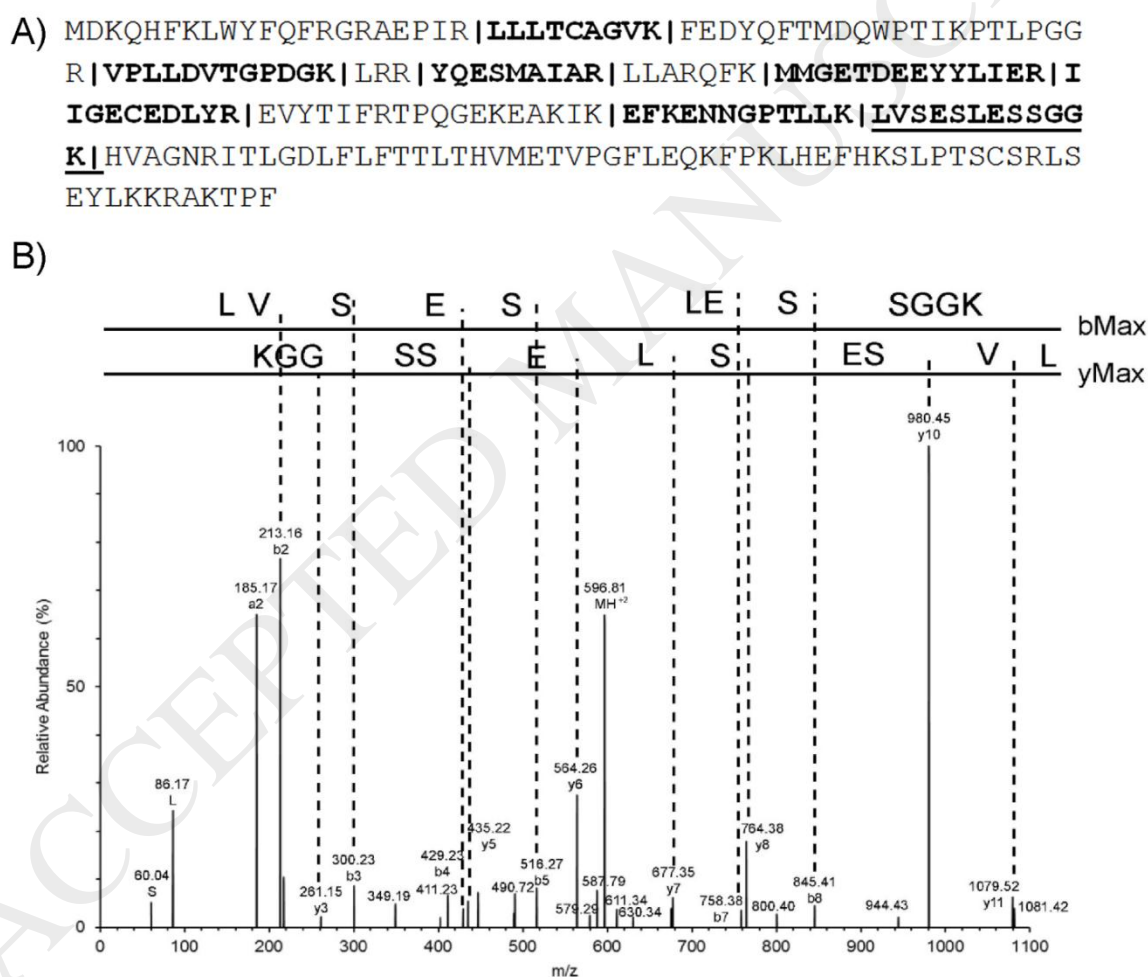
Figure 4. Confirmation of nFhGSTS1 via MSMS. A) Protein sequence of nFhGSTS1 accession no. 2WB9_A. Highlighted in bold are the seven identified peptides during MSMS including the characteristic peptide of this GST (bold and underlined) which is highlighted in
