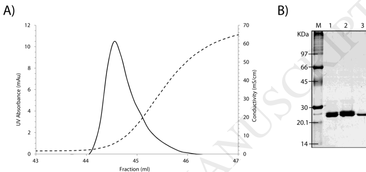
Figure 1. Purification of Fh GSTs1. A) The elution profile of protein bound to CM-Sepharose equilibrated to pH 6.8. Removal of protein from the column was achieved through a single step increase in NaCl concentration, shown by the increase in conductivity (dashed line). B) 1D SDS-PAGE gel stained with colloidal Coomassie showing different stages of purification, 1) GSH-affinity purified protein, 2) Cationic exchange unbound flow through protein, 3) CM-Sepharose purified protein
