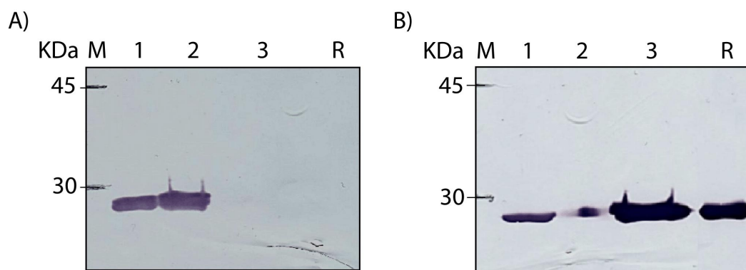
Figure 2. Western blot analysis of the different stages of nFhGSTS1 purification, developed using NBT/BCIP system. A total of 2 \mu g of protein was loaded onto each lane. 1) GSH-affinity purified GSTs 2) CM-Sepharose unbound flow through 3) CM-Sepharose purified R) recombinant FhGSTS1 control. A) Membrane probed with anti-mu class antibodies (1:5000 dilution). B) Membrane probed with anti-sigma class antibodies (1:30,000).
