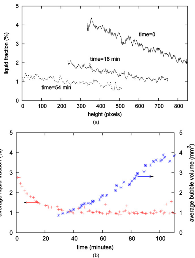
Fig. 5. (a) Vertical profiles of liquid fraction in the experimental foam at three different times, showing that the foam gets drier. (b) The evolution of the average liquid fraction of the foam, \langle \phi_l \rangle , and average bubble volume, \langle V_b \rangle , versus time.
