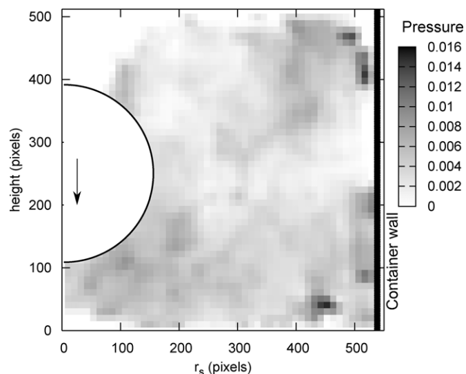
Fig. 6. 2D visualization of bubble pressure for a single image of the foam at 50 min: bubble pressure (with units \gamma (pixels) ^{-1} ) is mapped over (r_s, z) , where r_s denotes the radial distance from a vertical axis intersecting the sphere's centre and z denotes the height in the 3D image. The semi-circle shows the downward-moving sphere and the thick vertical line on the right represents the cylinder wall.
