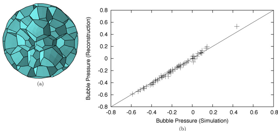
Fig. 3. (a) The reconstruction algorithm is applied to this simulated monodisperse foam with N=64 bubbles in a spherical container. The outer faces have been removed. (b) Bubble pressures in the simulated and reconstructed monodisperse foam, with a correlation coefficient of R=0.998 .
