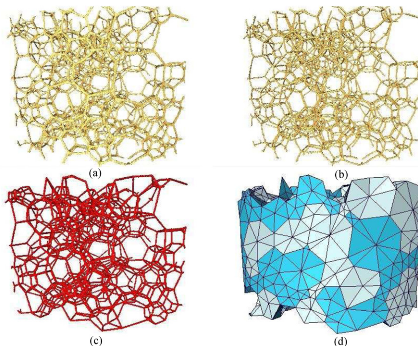
Fig. 1. Steps in the reconstruction algorithm: (a) Isolate the network of Plateau borders by filtering. (b) Skeletonize this binary image. (c) Extract the topology of the Plateau border network. (d) Reconstruct the films by finding cycles in the graph defined by the skeleton and define bubbles as the enclosed cells of this structure.
