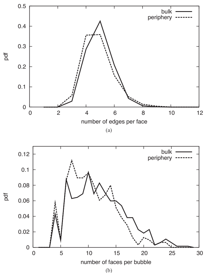
Fig. 4. Statistical information about the foam's topology at a time of 30 min, separated into 653 bubbles in the bulk and 315 peripheral bubbles: (a) the number of edges per face, n , and (b) the number of faces per bubble, F .
