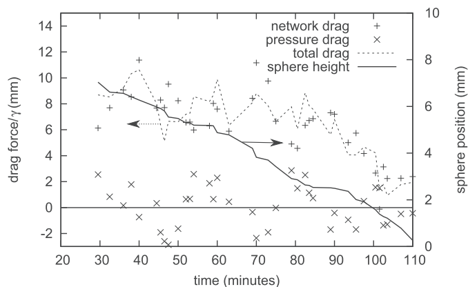
Fig. 7. Variations in the network, pressure, and the total drag force on the sphere, shown alongside its vertical position, versus time.
